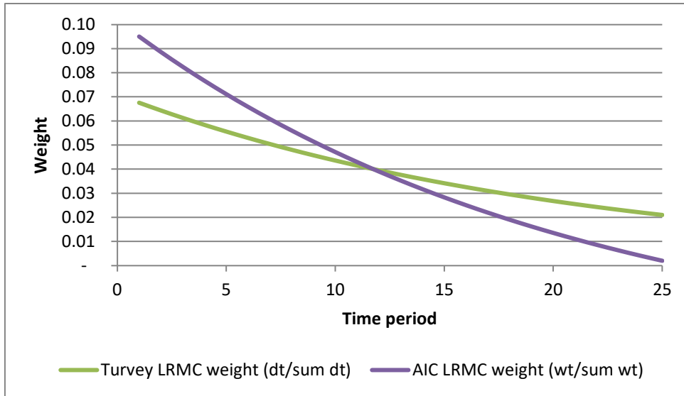
Figure 5: Comparison of Turvey and AIC weights
